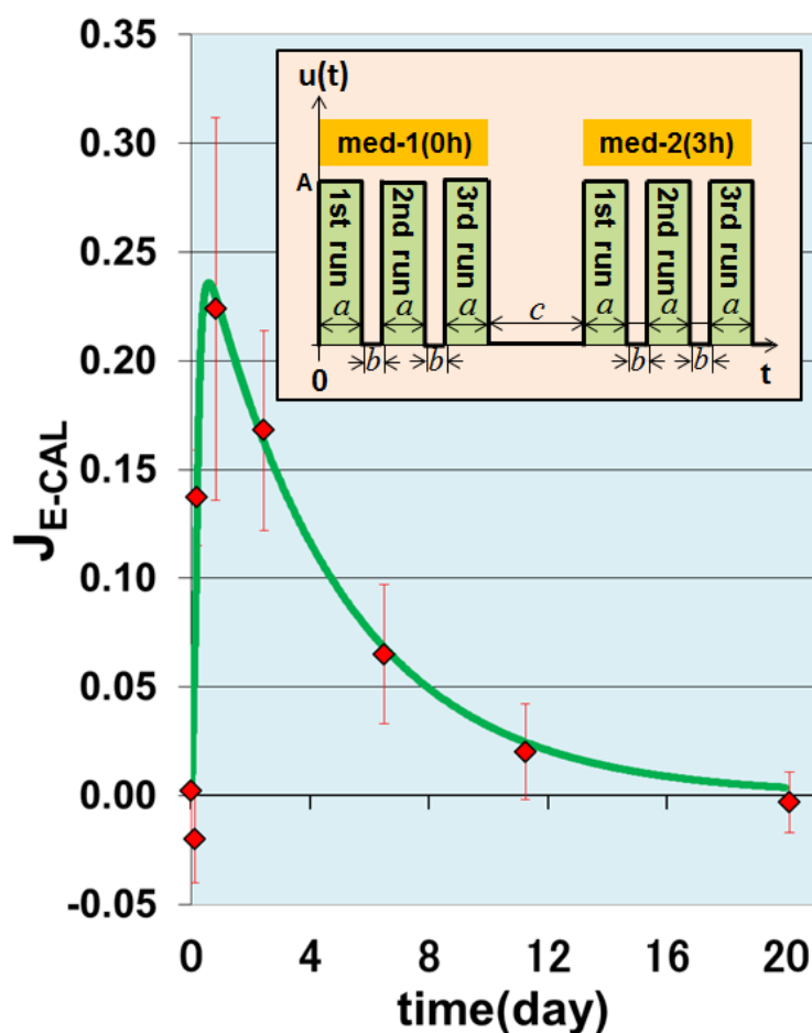
Fig. 4. Experimental results and theoretical curve for anomalous non-contact effect with a delay
